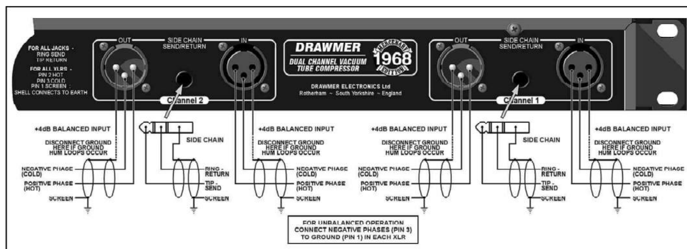
fig.1 1968 WIRING
